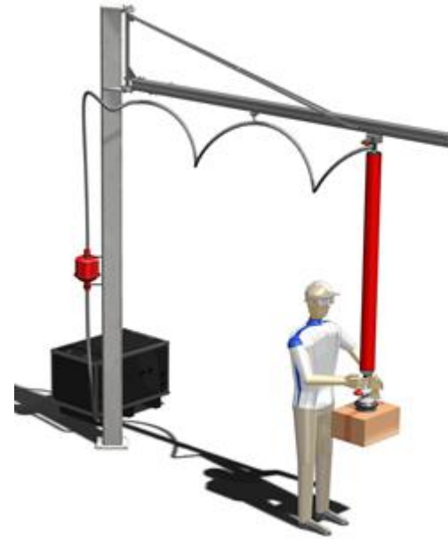
Pillar mounted
