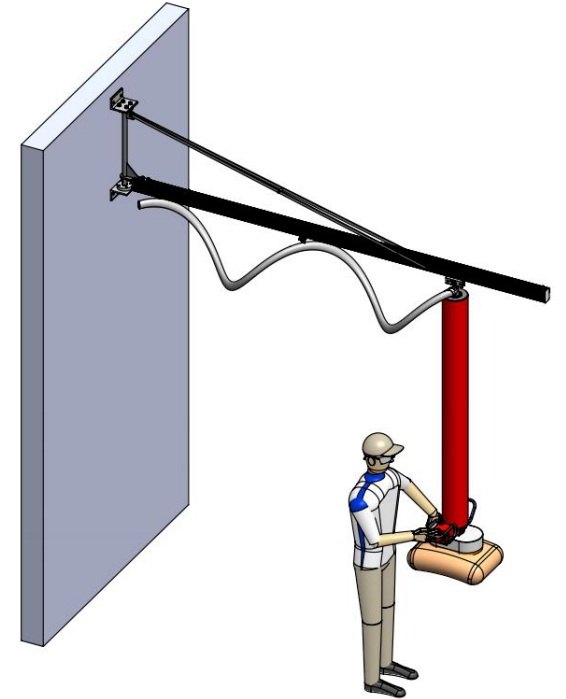
Wall mounted
